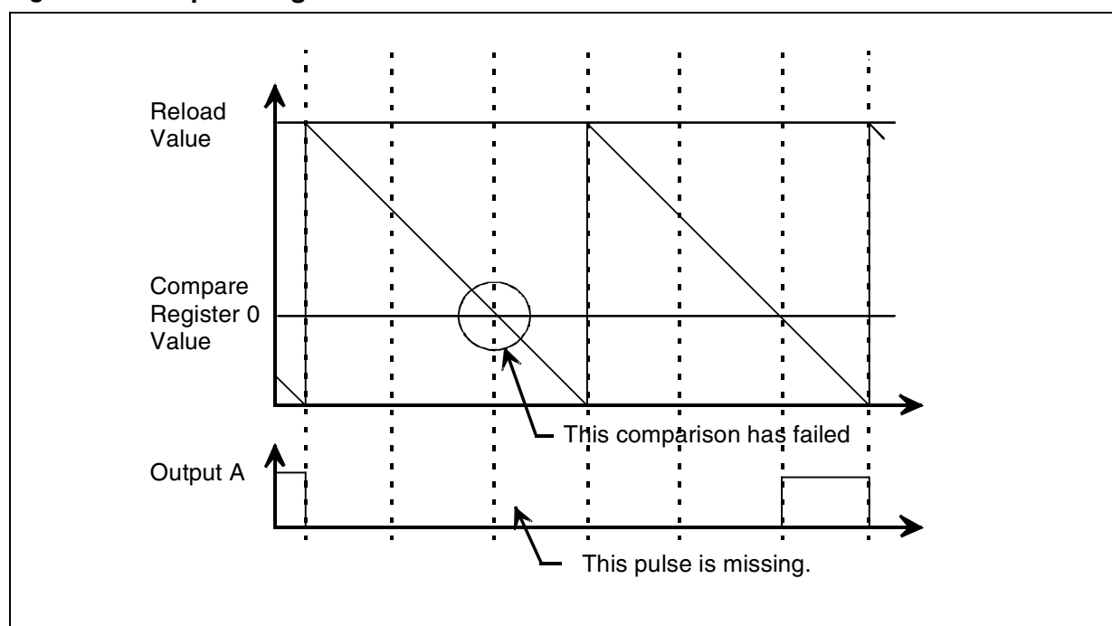
Figure 40. Compare Register is modified while its Content matches Counter
