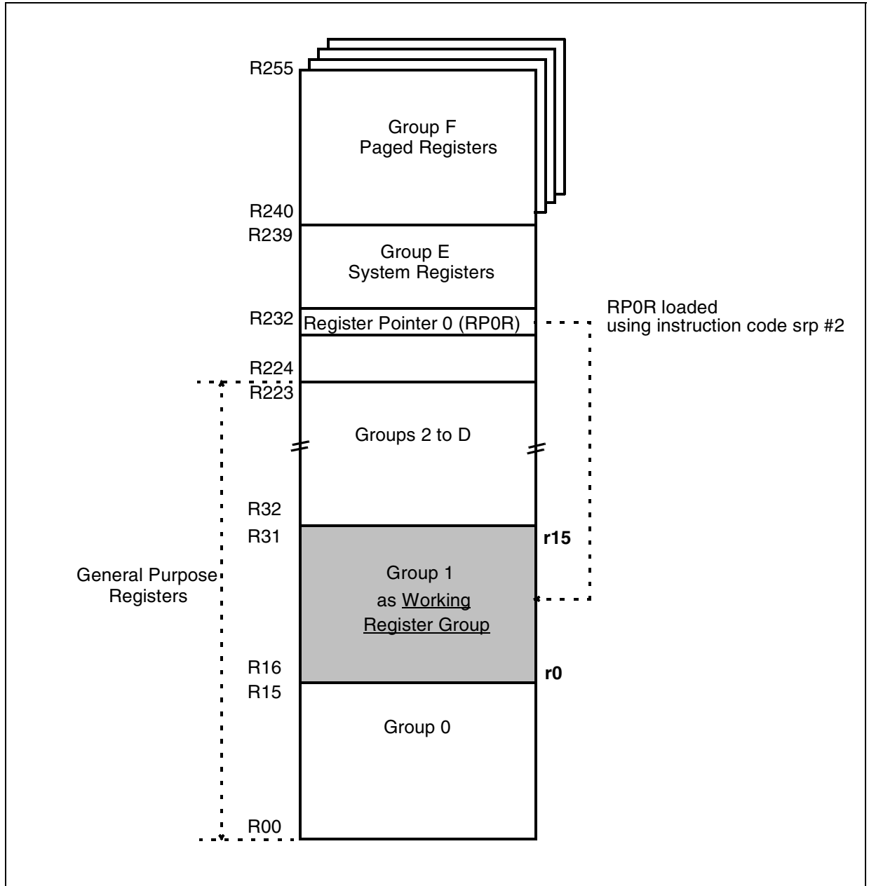
Figure 5. Selecting a 16-Register Working Group
