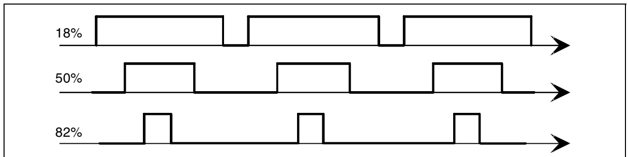
Figure 41. Symmetrical PWM Waveforms
