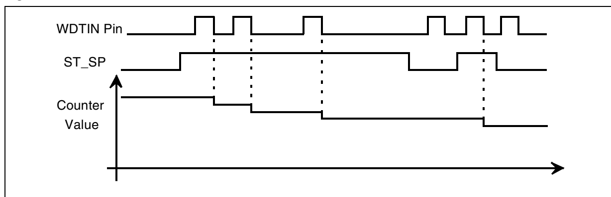
Figure 26. Timer in Event Counter Mode
