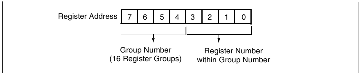
Figure 4. Register Group Addressing Scheme
