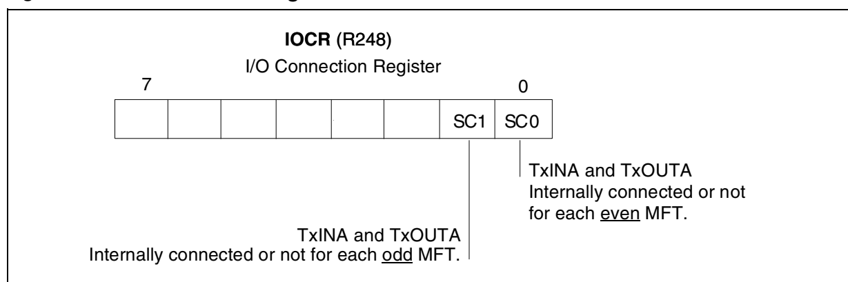
Figure 37. MFT I/O Control Register
