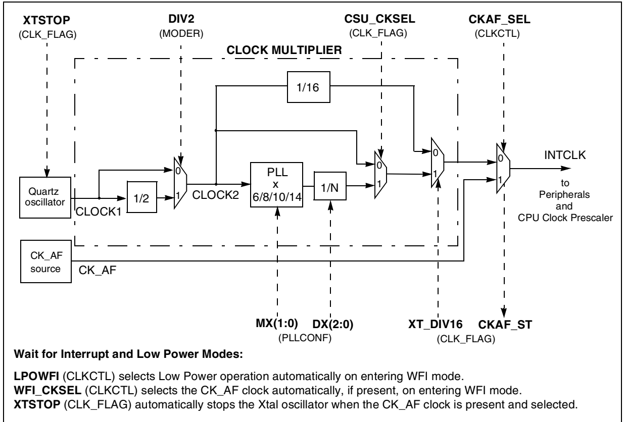
Figure 24. Clock Control Unit Programming
