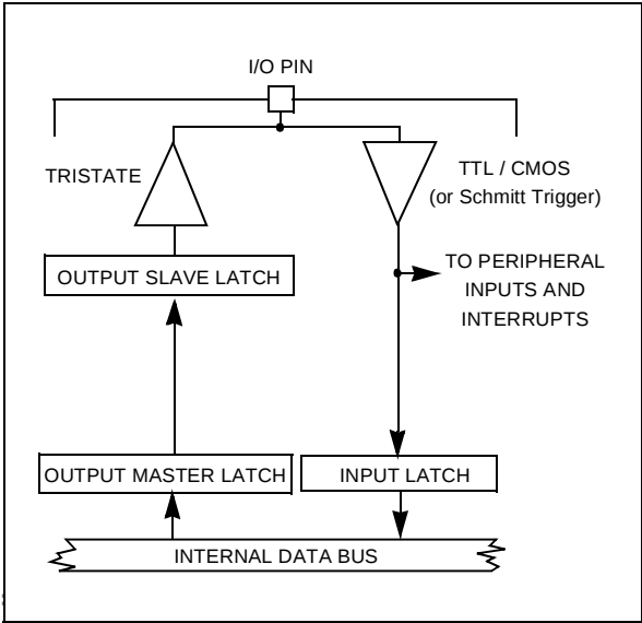
Figure 51. Input Configuration
