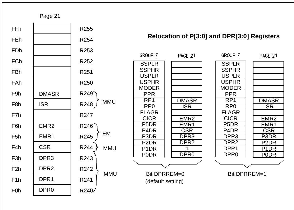
Figure 13. Page 21 Registers
