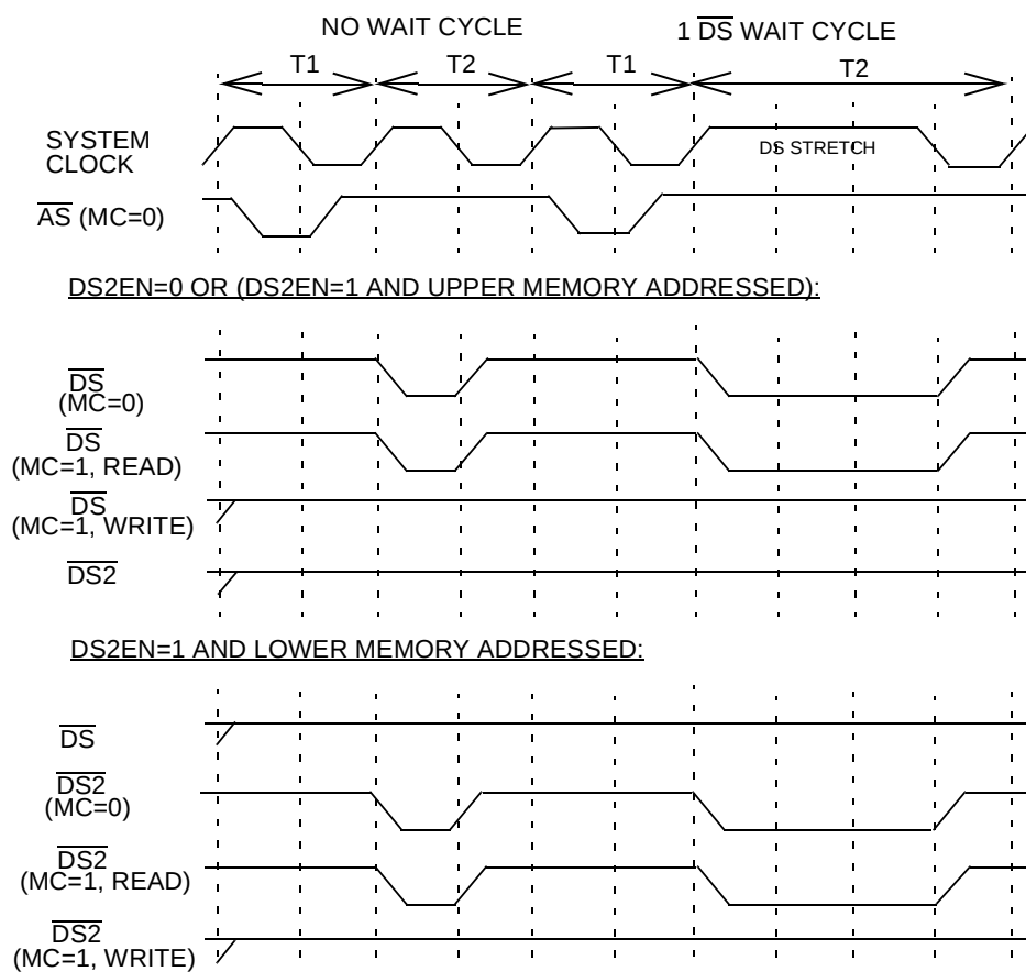
Figure 45. Effects of DS2EN on the behavior of \overline{DS} and \overline{DS2}
