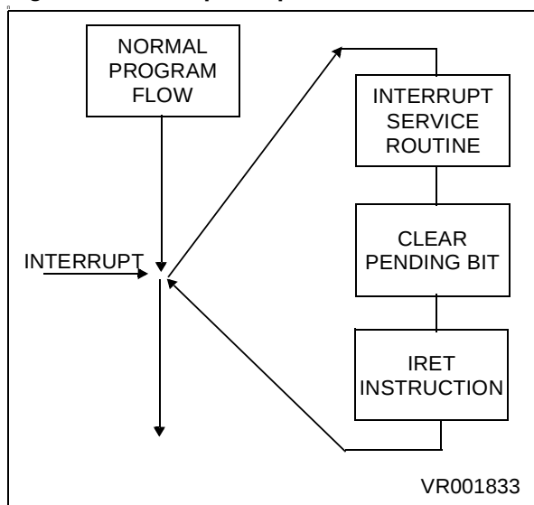
Figure 19. Interrupt Response
