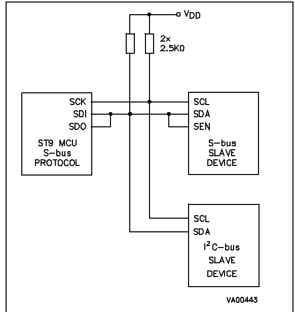
Figure 68. S-Bus / I 2 C-bus Peripheral Compatibility without S-Bus Chip Select
