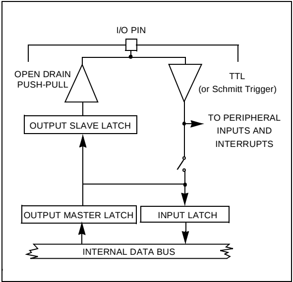
Figure 52. Output Configuration
