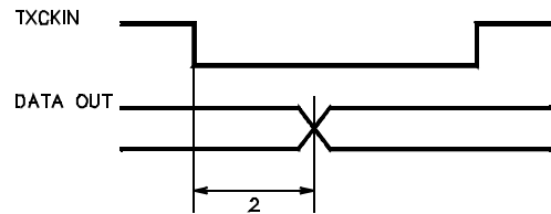
FIG 2: TRANSMISSION WITH EXTERNAL CLOCK 1X MODE
