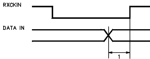
FIG 1: RECEPTION WITH EXTERNAL CLOCK 1X MODE
