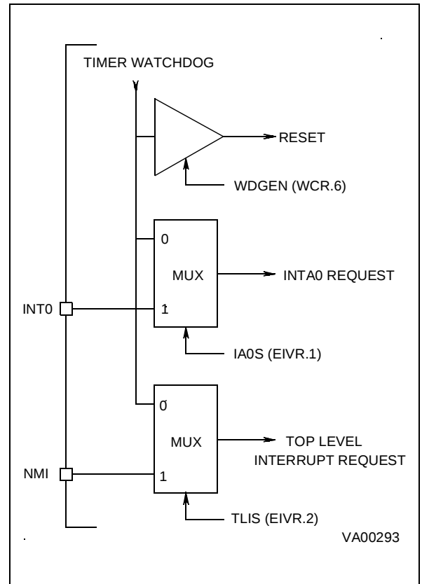
Figure 57. Interrupt Sources
