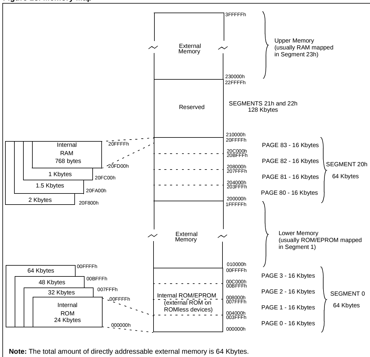
Figure 18. Memory Map
