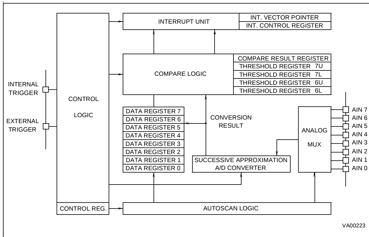
Figure 87. Block Diagram
