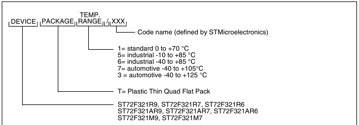
Figure 105. FLASH User Programmable Device Types
