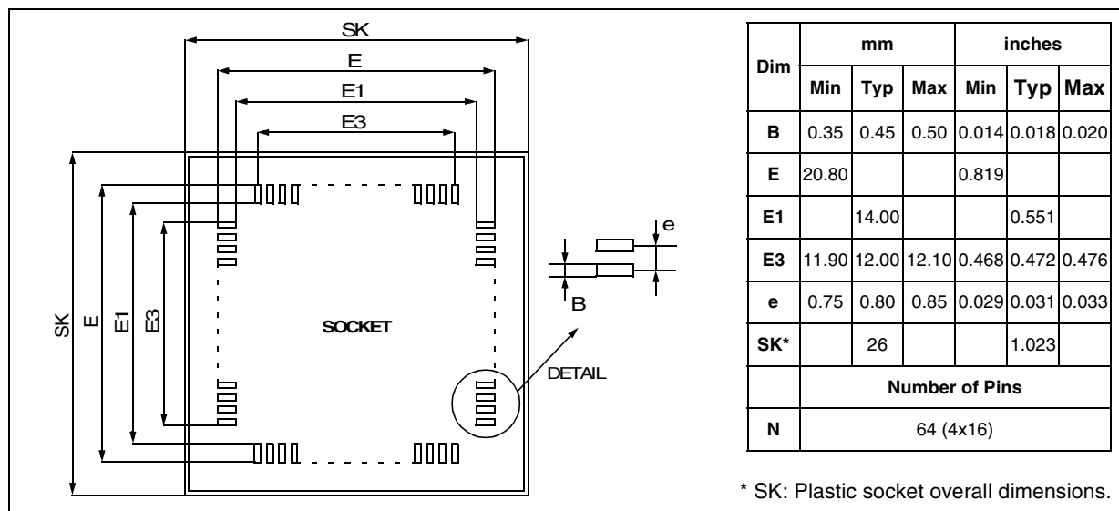
Figure 106. TQFP64 14x14 Device And Emulator Probe Compatible Footprint
