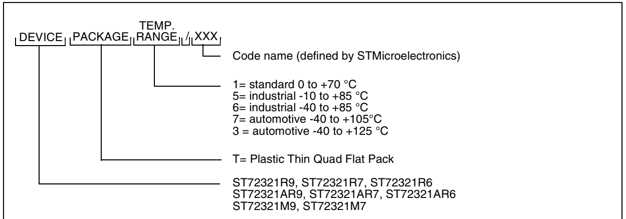
Figure 104. ROM Factory Coded Device Types
