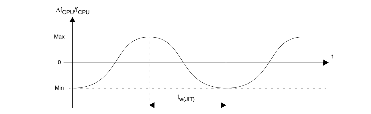
Figure 74. PLL \Delta f_{CPU}/f_{CPU} versus the time
