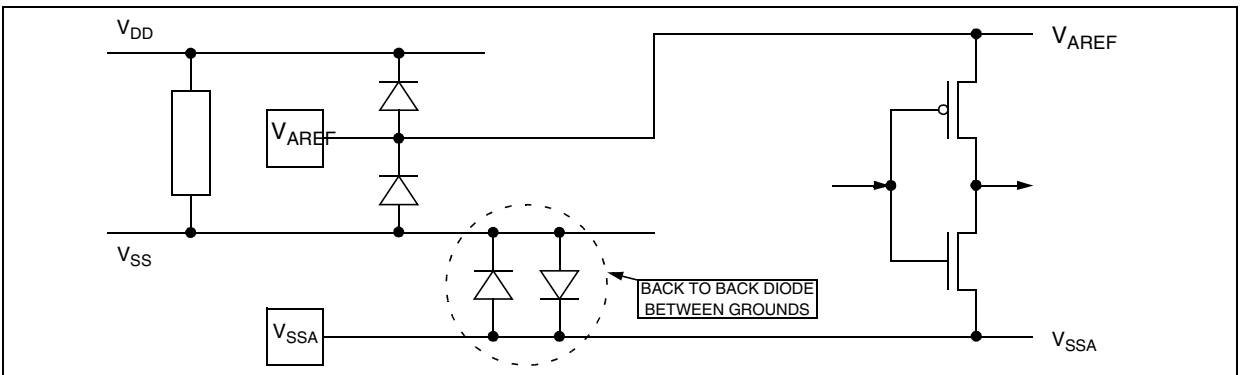
Figure 82. Multisupply Configuration
