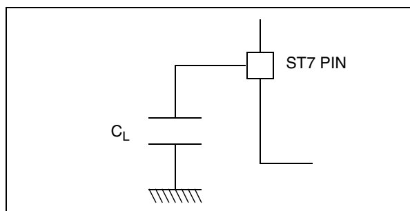
Figure 65. Pin loading conditions
