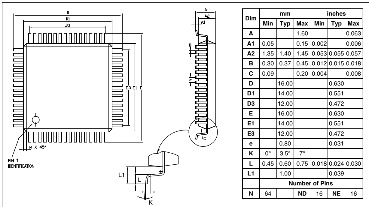
Figure 100. 64-Pin 14x14 Thin Quad Flat Package
