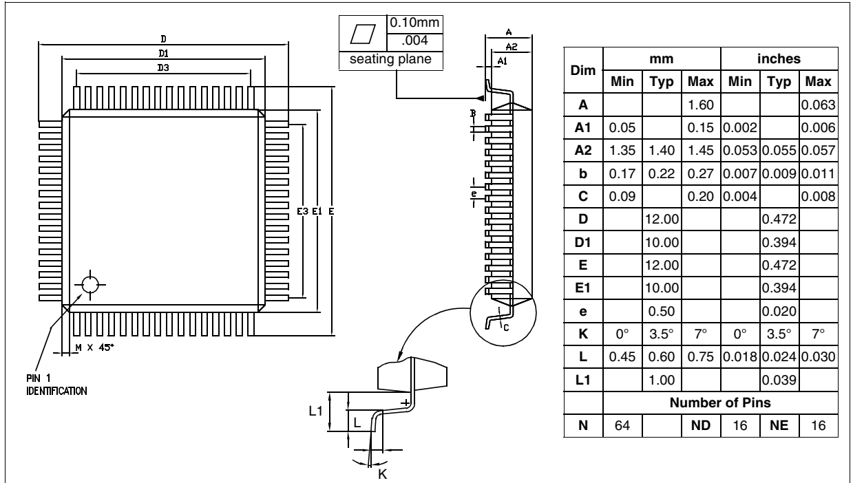
Figure 101. 64-Pin 10 x 10 Thin Quad Flat Package
