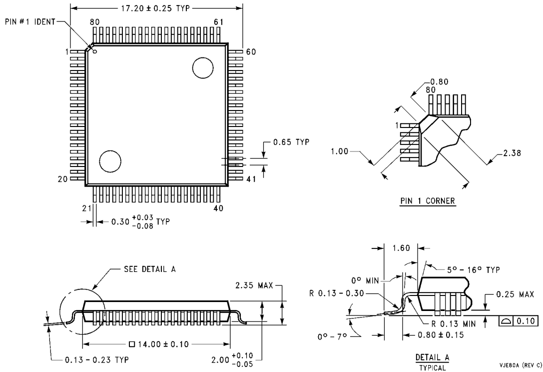
80 Lead Molded Plastic Quad Flat Package Order Number CR16MAR5VJExy See NS Package Number VJE80A
