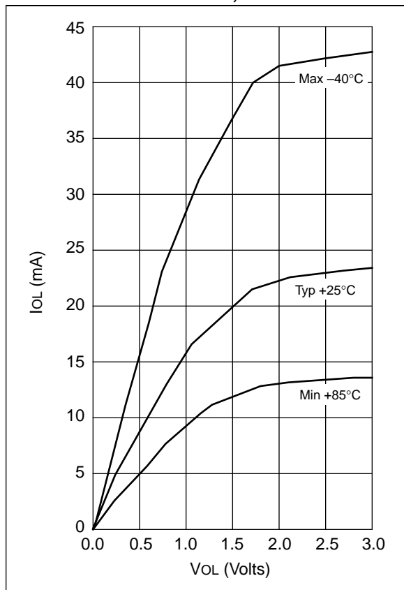
FIGURE 12-21: IOL vs. VOL, VDD = 3 V
