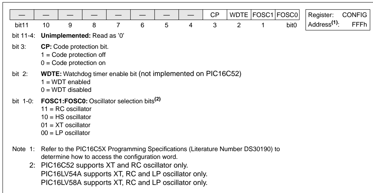
FIGURE 7-2: CONFIGURATION WORD FOR PIC16C52/C54/C54A/C55/C56/C57/C58A
