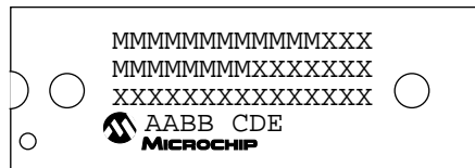
28-Lead PDIP (.600")
