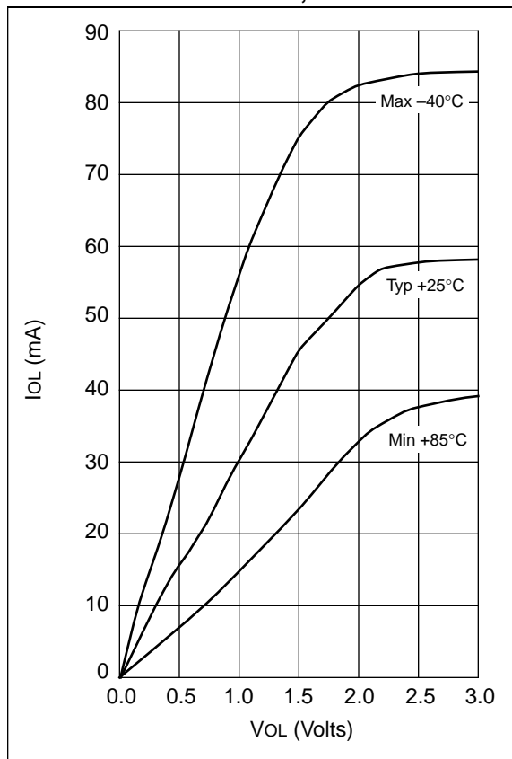
FIGURE 12-22: IOL vs. VOL, VDD = 5 V
