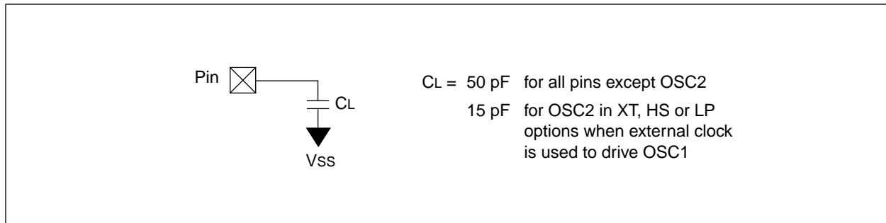
FIGURE 17-1: LOAD CONDITIONS - PIC16CR58A
