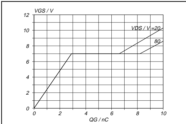
Fig. 13. Typical turn-on gate-charge characteristics. V_{GS} = f(Q_G) ; conditions: I_D = 11 A; parameter V_{DS}
